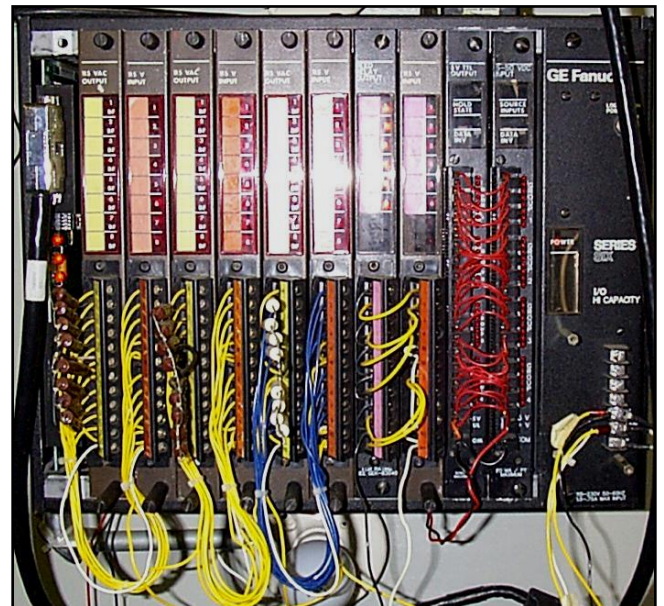
REMOTE I/O
