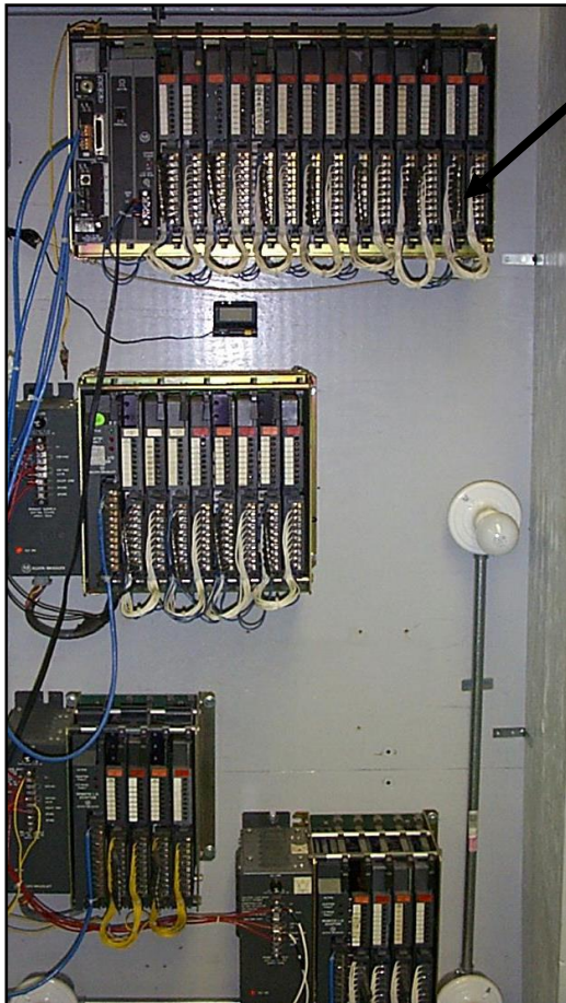
PLC 5 processor controlling multiple I/O racks.
