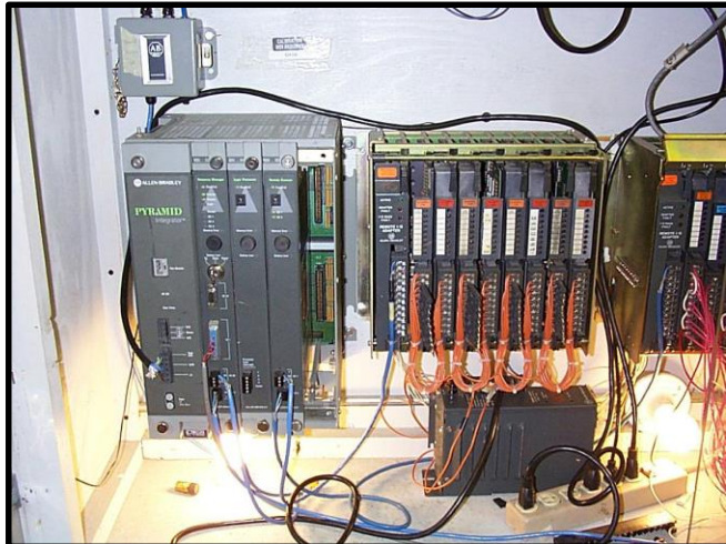
Pyramid system with integrated I/O shown in heat test cabinet.
