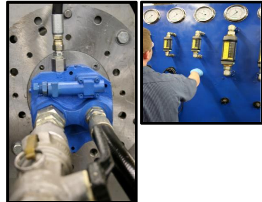
HYDRAULIC LOAD TEST STAND
