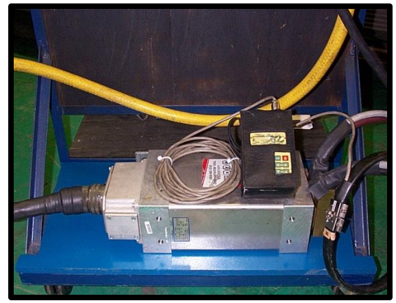
60KVA Weld Transformer
