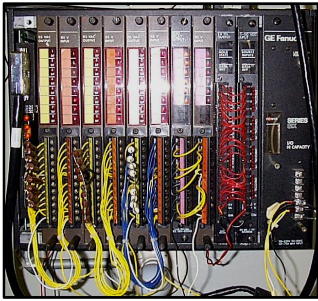
REMOTE I/O
