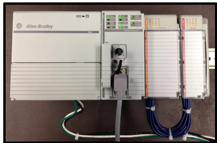
1769-L32E Compact Logix PLC
