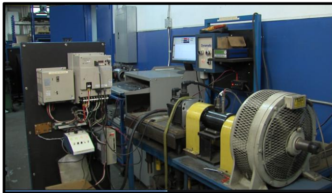
Eddy Current Load Stand
